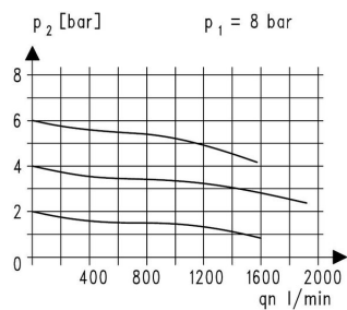
Flow diagram
