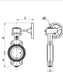
Sandwich mounting version
