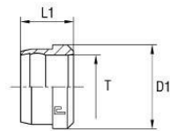
B3-Schneidring
