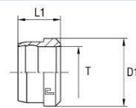
B3-Cutting ring
