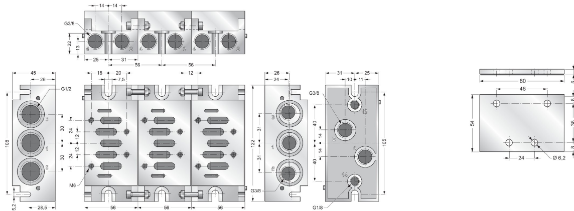
Connection fitting Typ BT12
