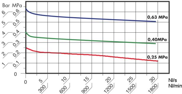
Indgangstryk = 10bar
